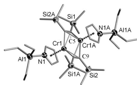
Figure 2. Molecular structure of 3 with thermal ellipsoids set at 50% probability. Hydrogen atoms are omitted for clarity. Selected bond lengths [Å] and angles [°]: Cr1–Cr1A 2.2992(15), Cr1–centroid 1.94(6), Cr1–C5 2.063(5), Cr1–C9 2.060(5), Cr1–C5A 2.075(5), Cr1–C9A 2.088(4), Al1–N1 2.015(4), C5–C9A 1.343(6), Si1–C5 1.875(5), C9–Cr1–C5 100.67(18), C9A–C5–Si1 140.1(4).
